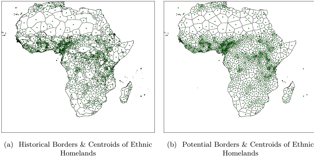
Figure 3: Historical Ethnic Borders, Centroids and Potential (Voronoi) Borders in Africa
